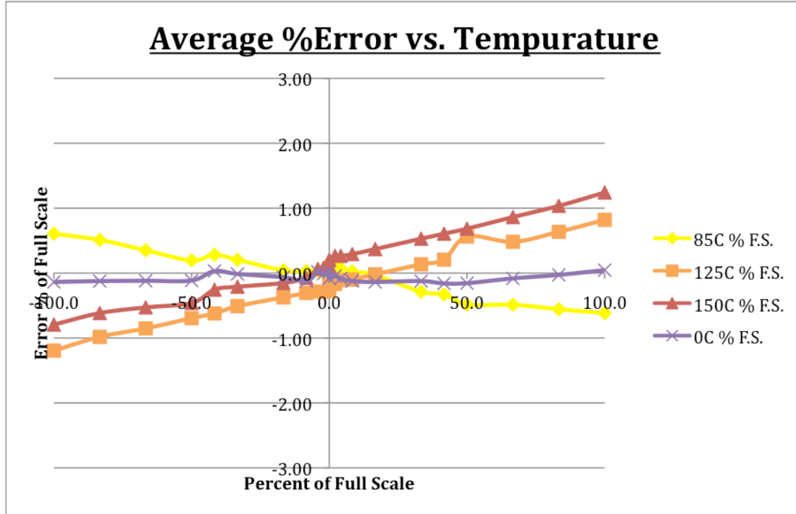
Error Plot
